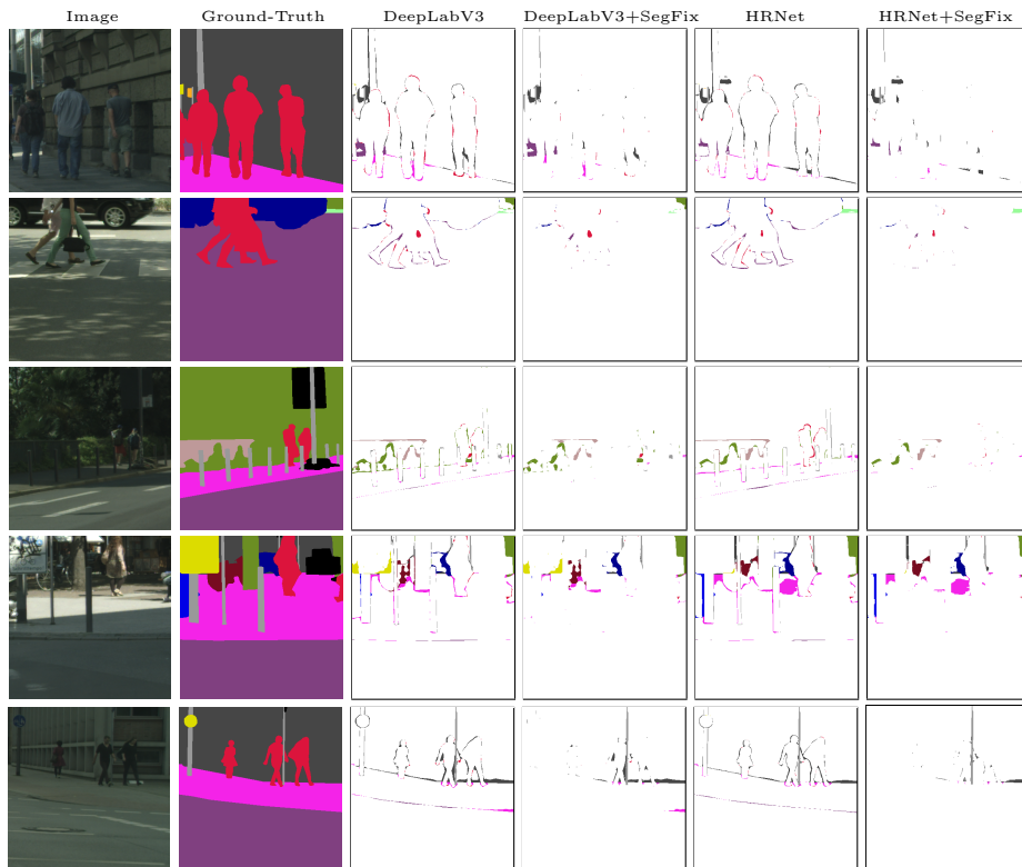
Fig. 9: Qualitative comparison in terms of errors on Cityscapes val. Our approach well addresses the existing boundary errors of various categories, e.g., person, pole and traffic sign, for both DeepLabv3 and HRNet.
